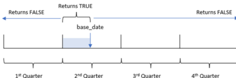
Diagram of inquartertodate function
