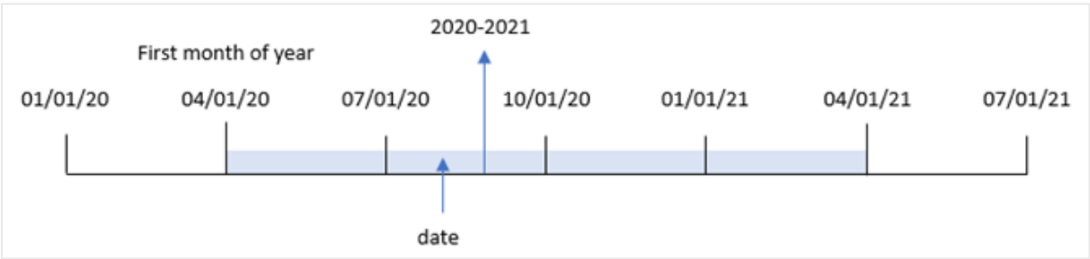
Diagram of yearname() function with April set as the first month of the year.
